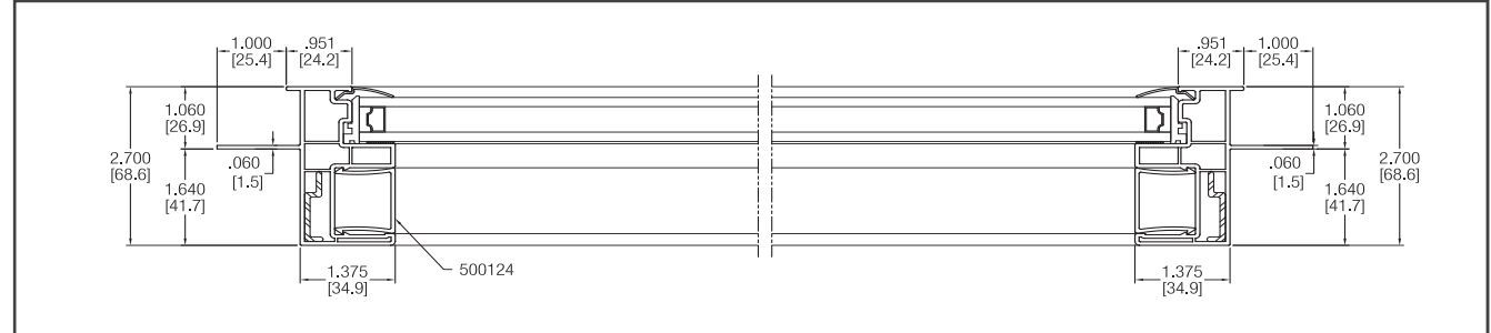
SECTION B-B
