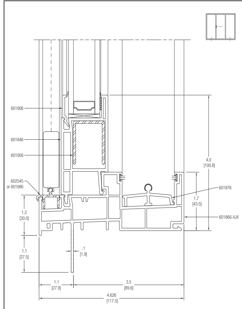
SILL FIXED
