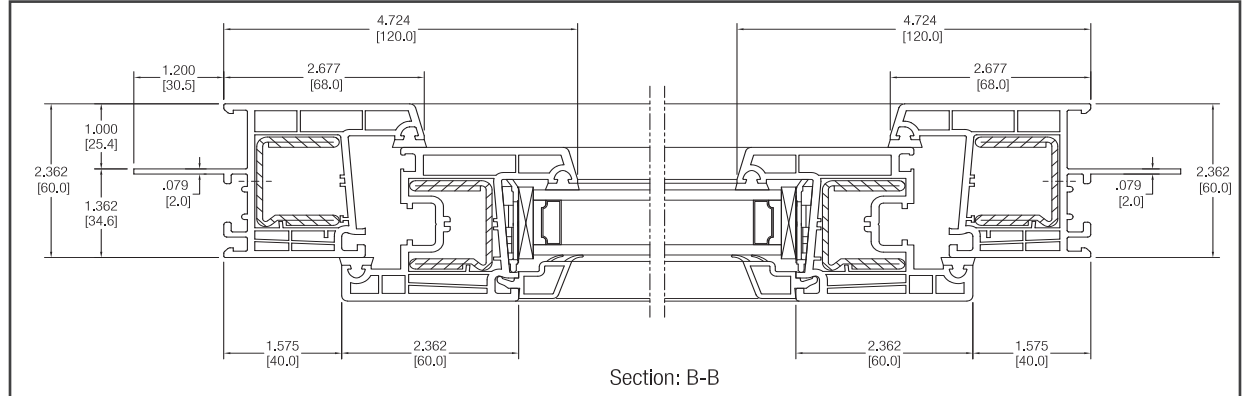
SECTION B-B
